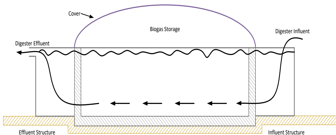
EXHIBIT 3-23: Plug Flow Anaerobic Digester System Diagram
