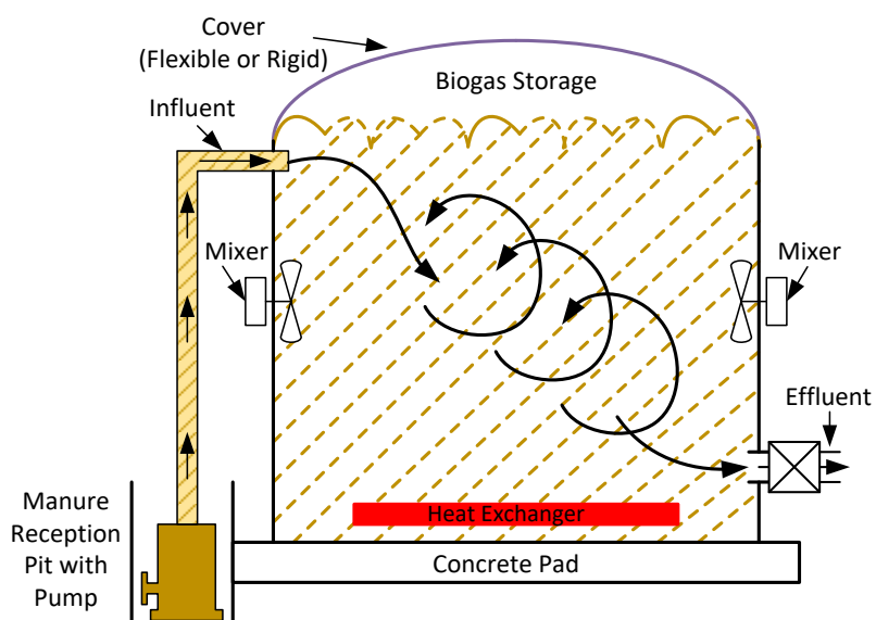
EXHIBIT 3-24: Complete Mix Anaerobic Digester System Diagram
