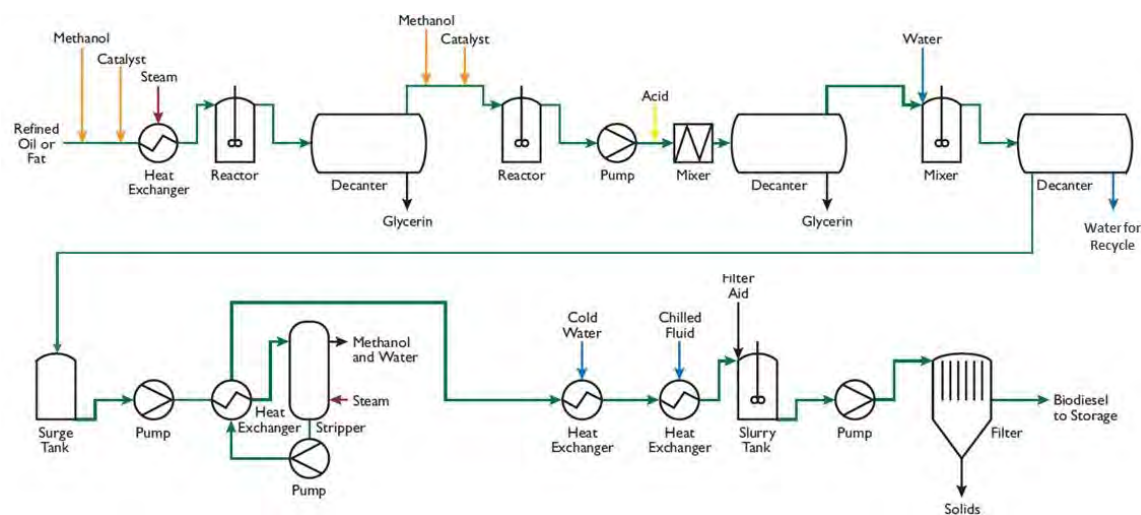
EXHIBIT 7-3: Transesterification Flow Diagram
