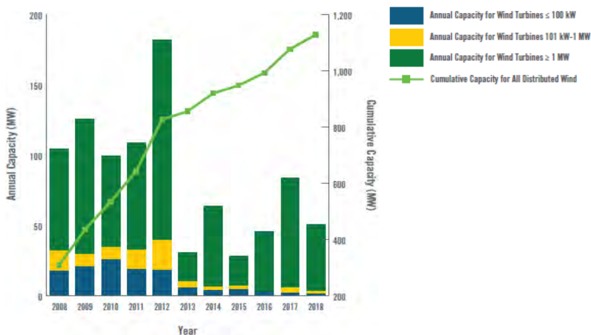
Figure 1. U.S. distributed wind capacity
