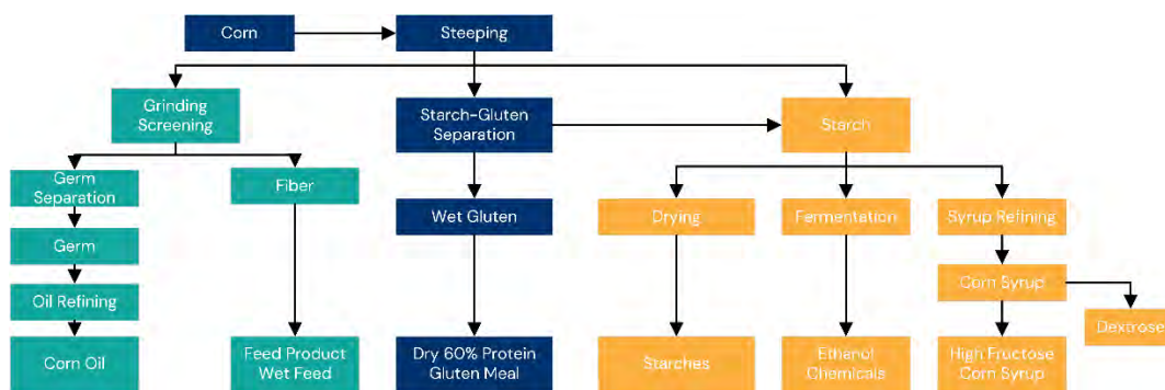
EXHIBIT 6-2: Wet Milling Process
