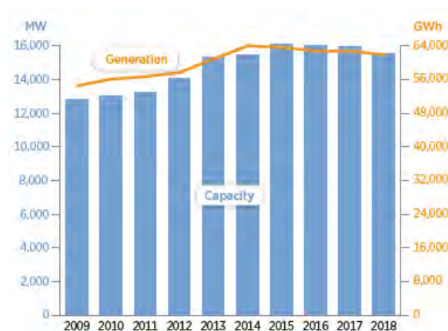
EXHIBIT 3-5: U.S. Bioenergy Power Generation Capacity and Annual Production Trends
