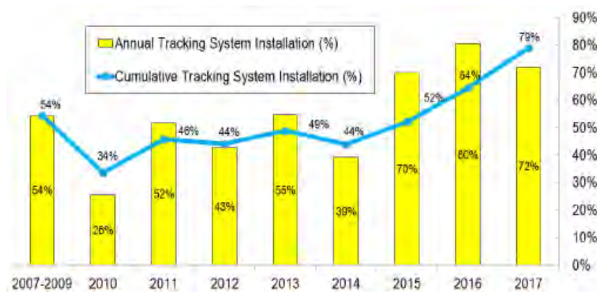
EXHIBIT 4-3: Prevalence of Single- or Dual-Axis Tracking Among Utility-Scale PV Systems
