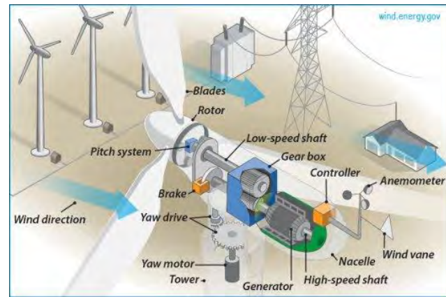
EXHIBIT 5-3: Rural Utility-Scale Wind Energy System in California
