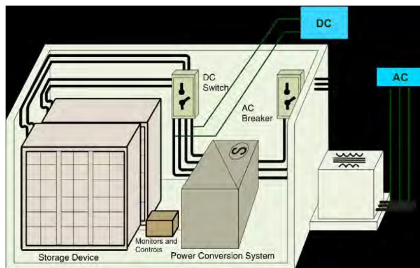
EXHIBIT 4-23: Basic Components of a Battery Energy Storage System
