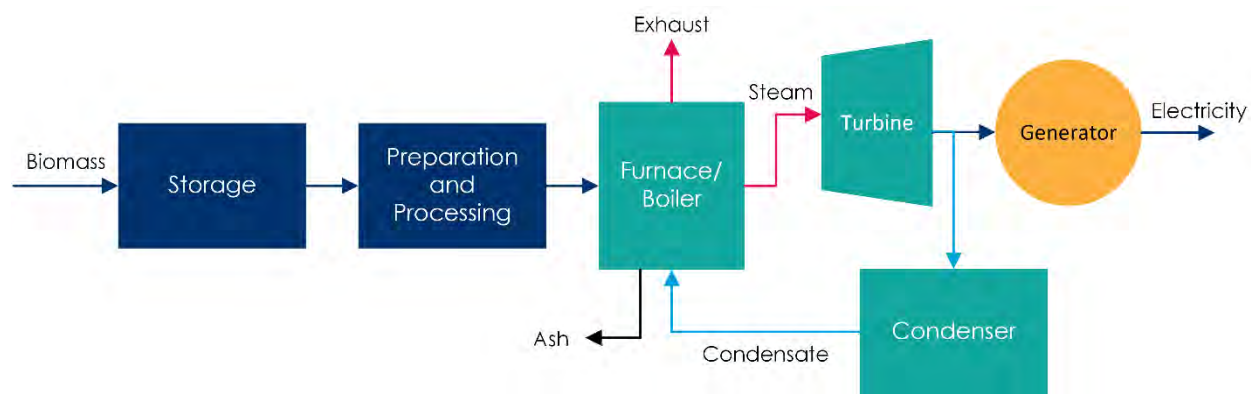
EXHIBIT 3-1: Combustion/Steam Turbine Biomass Power Generation Block Diagram
