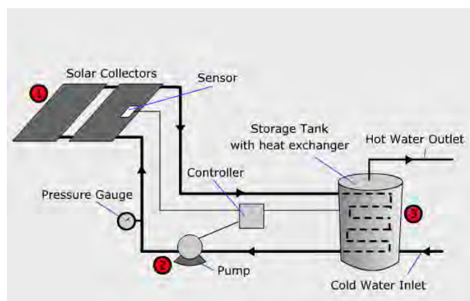
EXHIBIT 4-25: How a Typical Active Solar Water Heating System Operates
