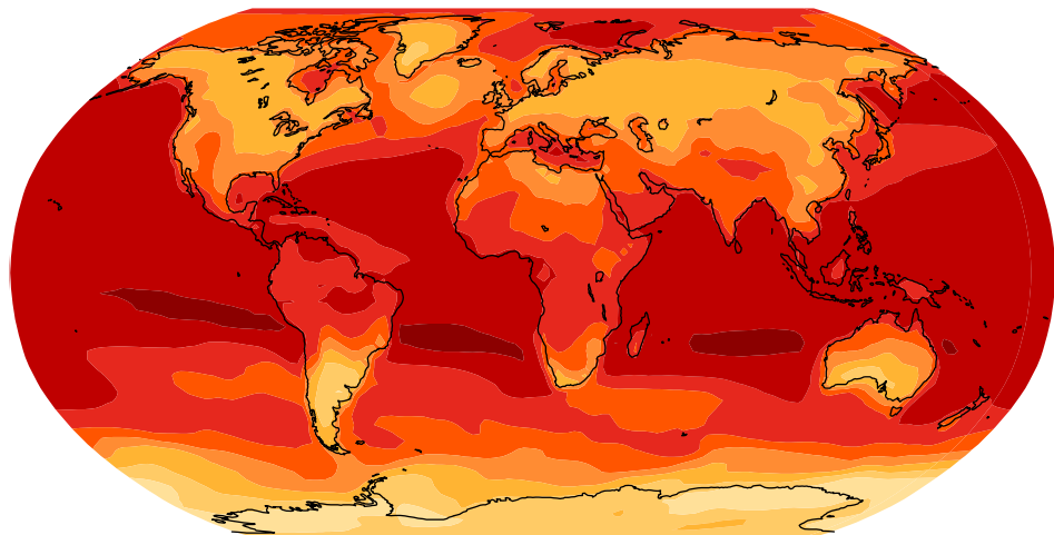
RCP8.5, 2081-2100 vs. 1986-2005
