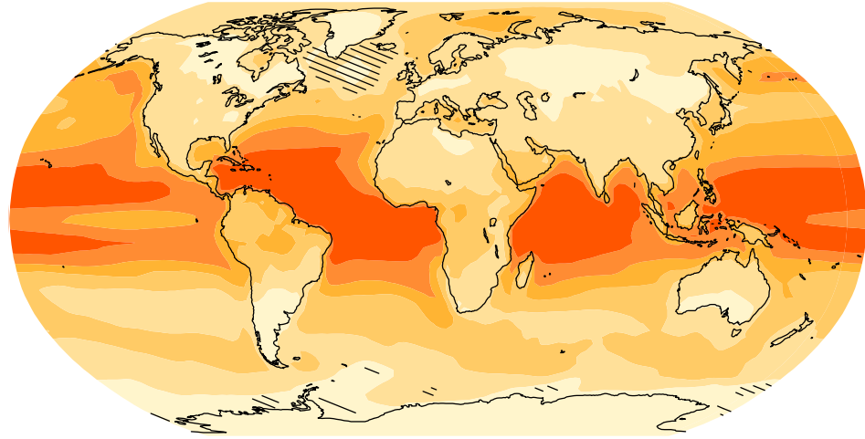
RCP2.6, 2081-2100 vs. 1986-2005
