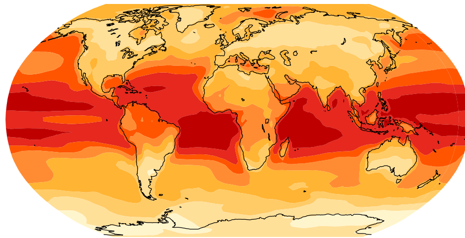
RCP8.5, 2046-2065 vs. 1986-2005
