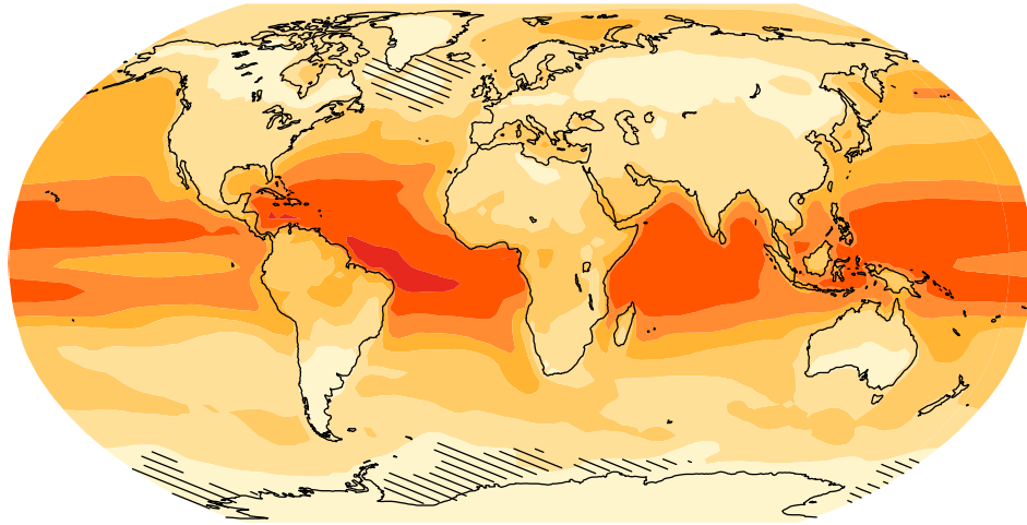
RCP2.6, 2046-2065 vs. 1986-2005
